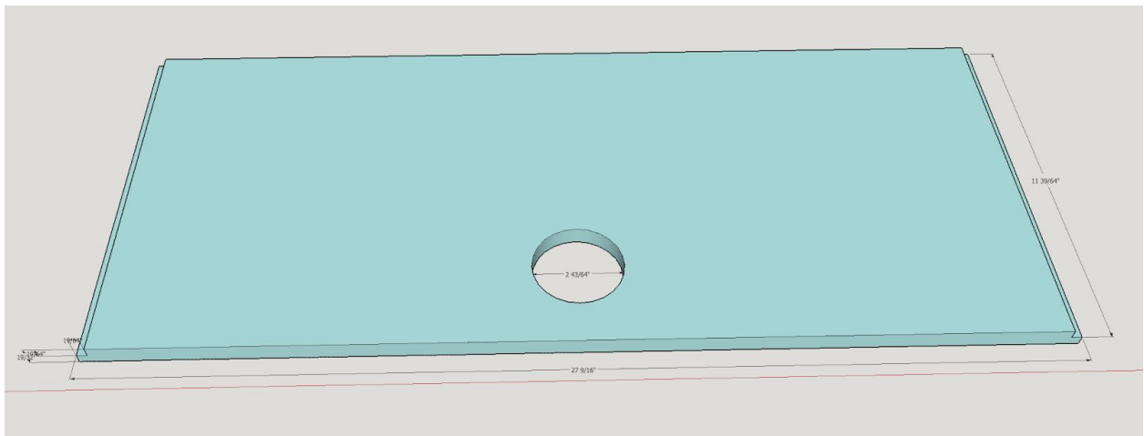
Back of back cabinet with hole for dust collection (make this larger if you want your saw to tilt)
