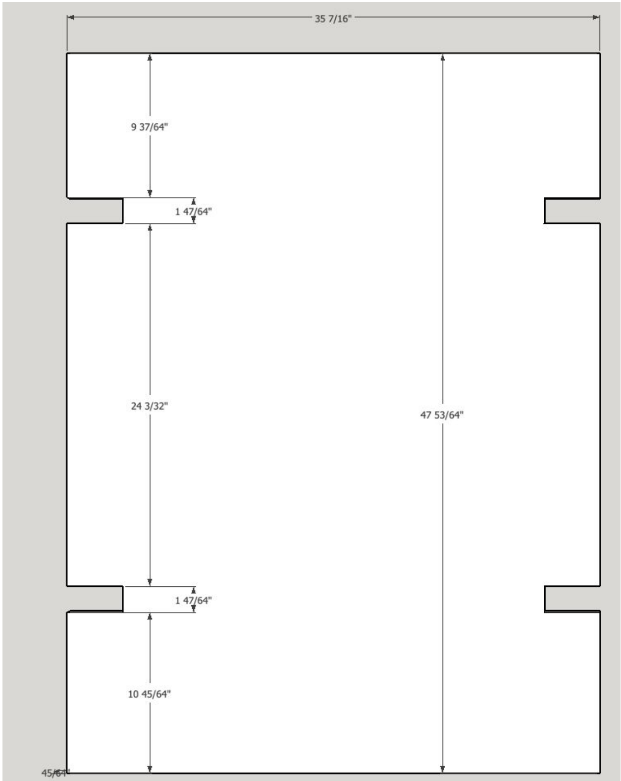
Bottom piece that goes on the lower frame. Holes are cut-outs for the frame.
