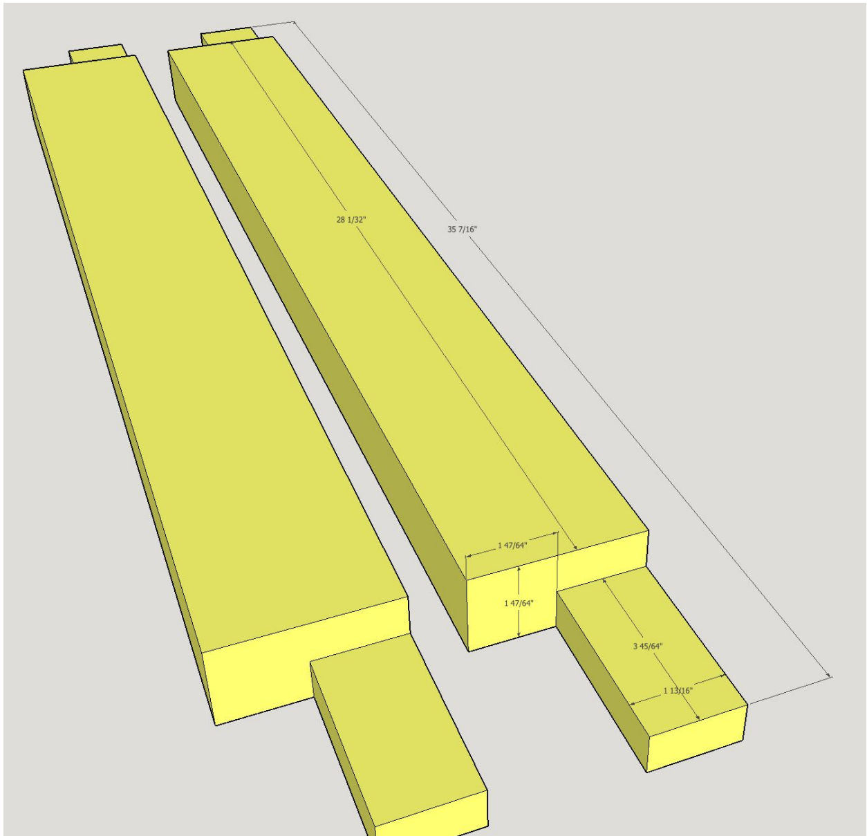
Pieces of the frame that lay horizontal on the uprights.
